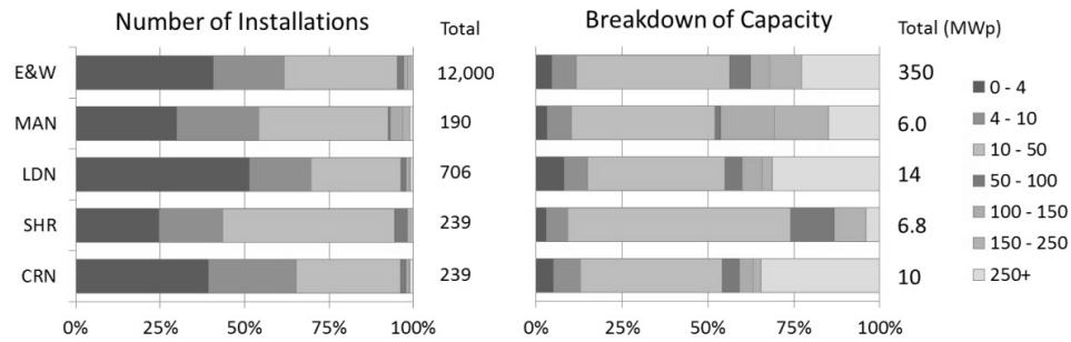
Fig. 9 – Breakdown of non-domestic PV installations by number and capacity (MWp)
