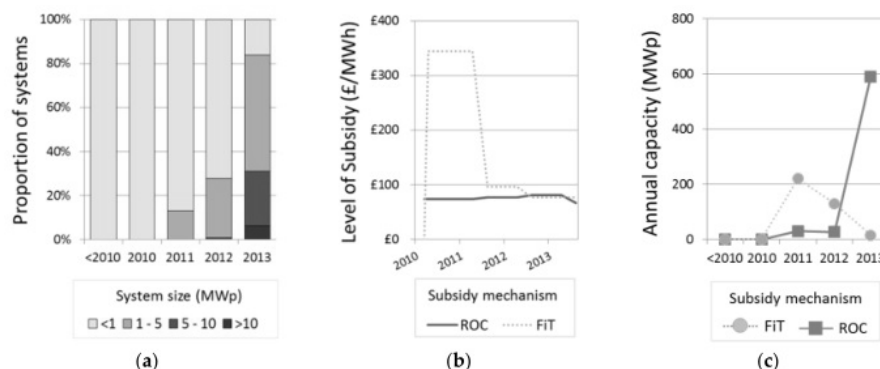
Fig. 4 – Annual ground-mount PV deployment by (a) system size; (b) level of subsidy and (c) deployment by subsidy type
