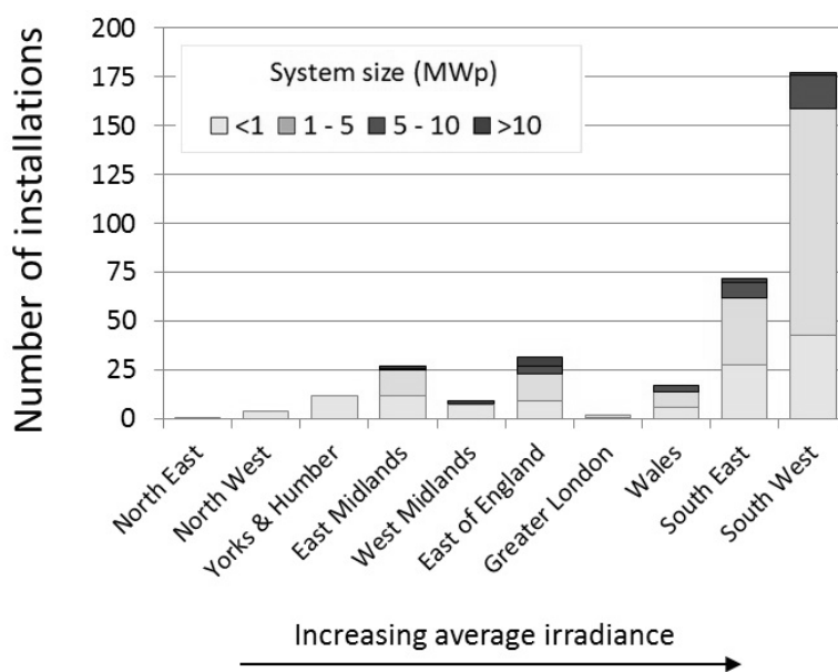
Fig. 12 – Regional installations of ground-mount PV by system size band (MW p )
