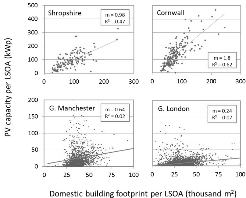
Fig. 6 – Domestic PV capacity against building footprint per lower-layer super output area (LSOA). Insets show gradient ( m ) and R-squared values
